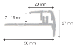
5 Stair nose aluminium (on request) Fits to flooring thickness of 7 - 16 mm, W = 23 mm, L = 2.7 m. PGSTPSILV, silver. Surface: aluminium.
